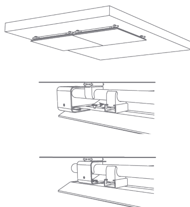
CEILING MOUNTING
