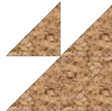
Azores TRG 90
