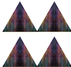
Azores TRG 60
